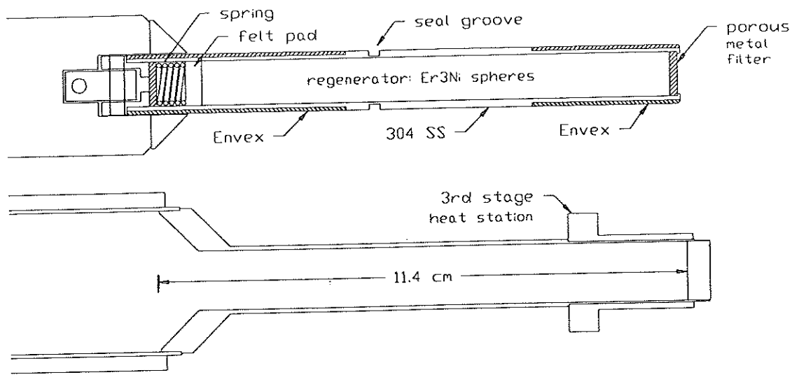
Fig 1. Cross sectional views of a 3rd stage cylinder and typical displacer.
