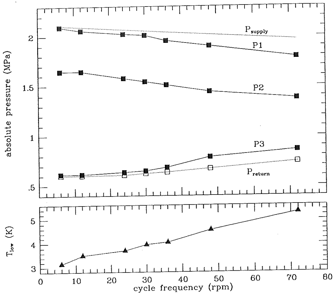
Fig. 8. (top panel) Helium pressures in the 3rd stage expansion volume, monitored at 7 different cycle frequencies; P_{\text{supply}} , P_1 , P_2 , P_3 , and P_{\text{return}} are measured as indicated in Figure 7. (bottom panel) Lowest 3rd stage temperature as a function of cycle frequency. (Refrigerator #3, 2.54 cm stroke, 45 g \text{Er}_3\text{Ni} , clearance seal.)
