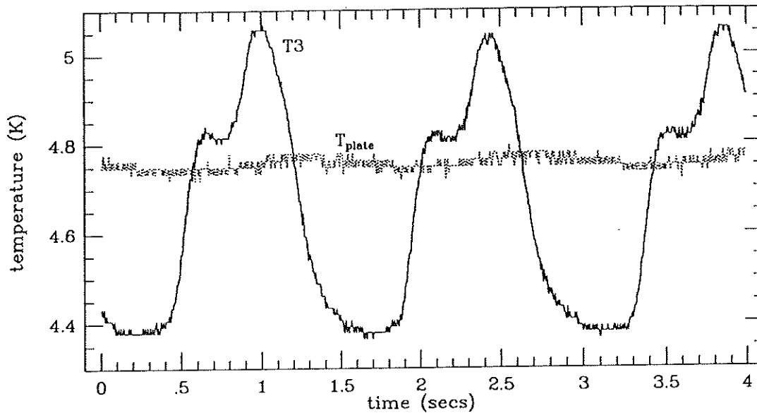
Fig 9. Temperature swing measured directly on the 3rd stage (T3) and on a plate thermally loaded with 10 g of \text{Er}_3\text{Ni} powder ( T_{\text{plate}} ). The cycle frequency is 42 rpm.
