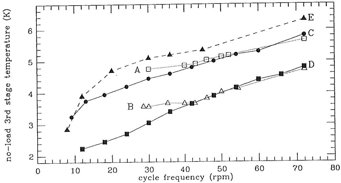
Fig. 3. No-load temperature vs. cycle frequency for 5 different displacers: A - refrigerator #1, 46 g of 350 micron diameter Pb spheres, 1.9 cm stroke, clearance seal; B - refrigerator #1, 30 g \text{Er}_3\text{Ni} , 1.90 cm stroke, clearance seal; C - refrigerator #2, 57 g \text{Er}_3\text{Ni} , 2.54 cm stroke, CTI seal; D - refrigerator #2, 53 g \text{Er}_3\text{Ni} , 3.18 cm stroke, CTI seal; E - refrigerator #3, 46 g \text{Er}_3\text{Ni} , 2.54 cm stroke, clearance seal.
